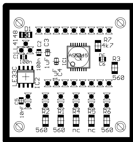
Layout: Bottom Components
